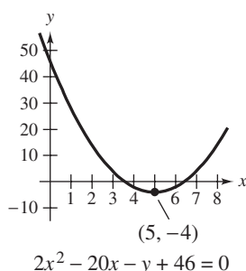
103. Parabola
