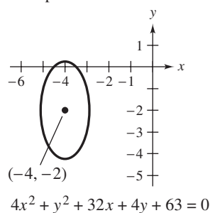
105. Ellipse
